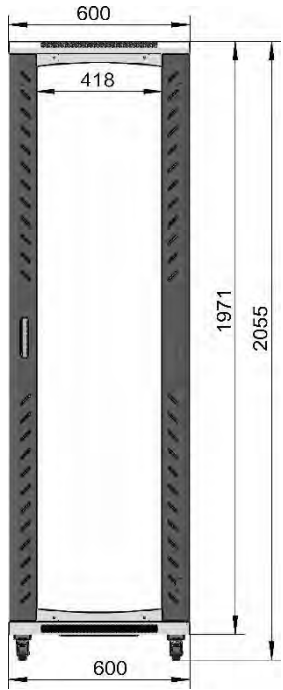
Front(Toughened glass)
